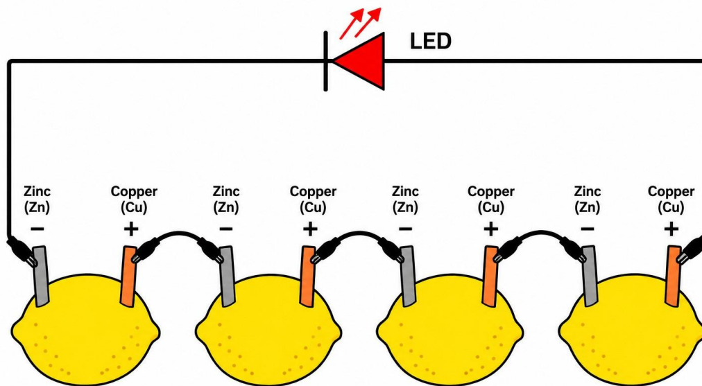
Schematic overview of the Lemon Battery.
